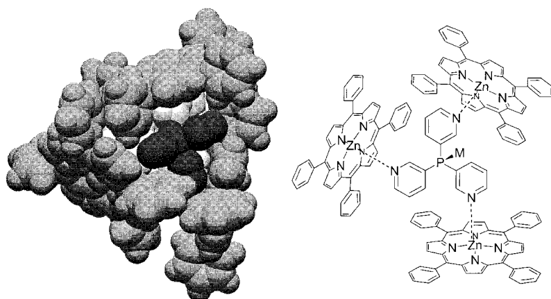
Figure 1. Modeled structure of an encapsulated transition metal catalyst consisting of porphyrin 1 (gray), tris( m -pyridyl)phosphane ( 4 ) (white) and \text{M} = [\text{RhH}(\text{CO})_3] (dark gray).
